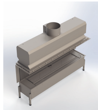
FREEDOM 3 SIDES PANORAMA
